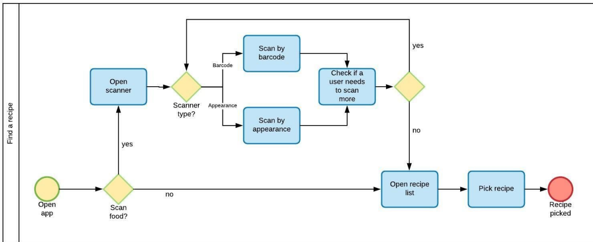
2. Find a recipe flowchart diagram
