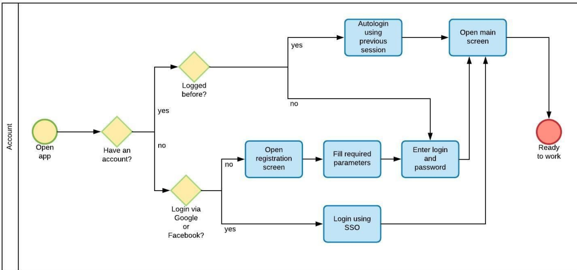
1. Account flowchart diagram
